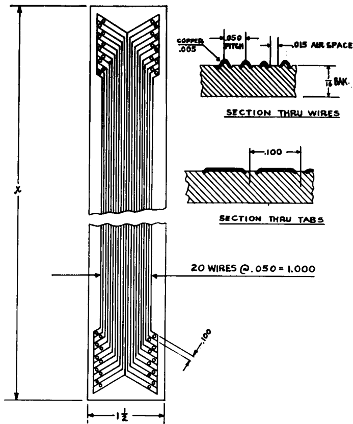
FIGURE 14.3. Die-stamped wire panel for replacing conventional cables.
