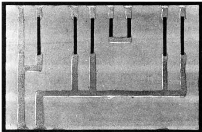
FIGURE 7.3. Two stage amplifier unit incorporating four capacitors as a part of the base plate.
