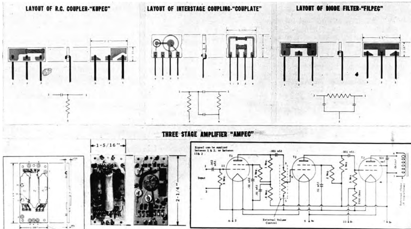
FIGURE 2.1. Examples of techniques used in printed circuits.
