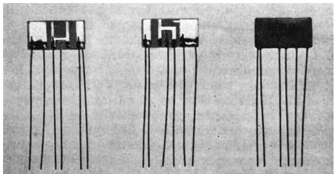
FIGURE 17.6. Herlec "Bulplates," showing construction. The unit at the right is coated with a thermosetting material.
