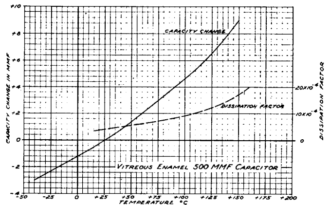
FIGURE 7.5. Graphs showing capacity vs. temperature and loss vs. temperature of vitreous dielectric capacitors.
