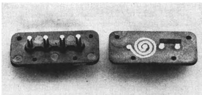
FIGURE 17.4. Printed plug-in unit on a molded Mycalex base plate.
