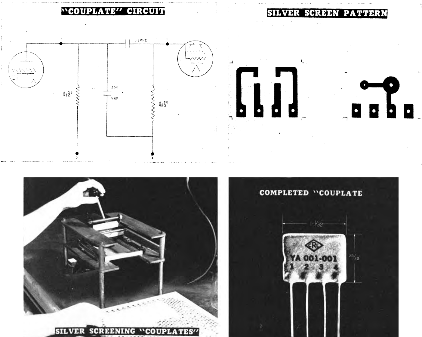
FIGURE 2.2. Steps used in manufacturing the "Couplate."
