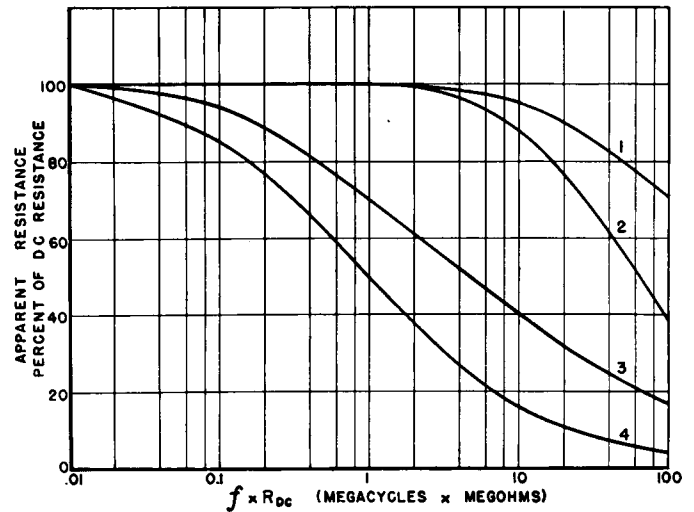
FIGURE 4.6. Frequency characteristics of different types of resistors.
