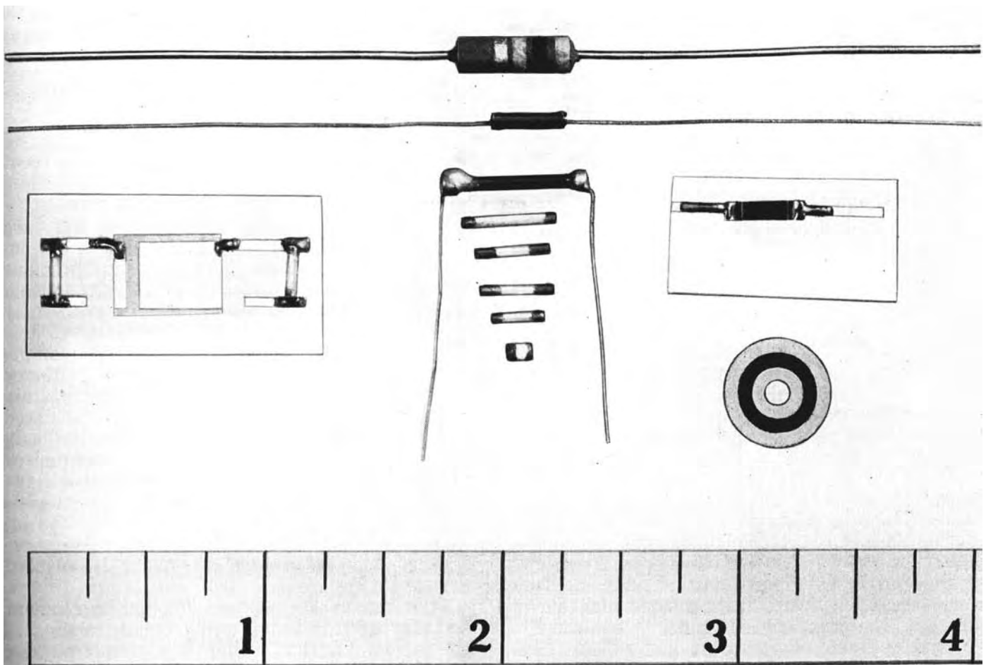
FIGURE 16.1. Reading down (center): Commercial \frac{1}{4} watt resistor; Balcohm hermetically sealed axial lead resistor; Balcohm hermetically sealed radial lead resistor; resistors with body ends tinned for direct soldering.
