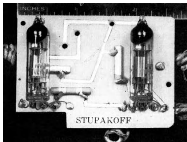
FIGURE 17.1. Production model of two-stage printed circuit amplifier.
