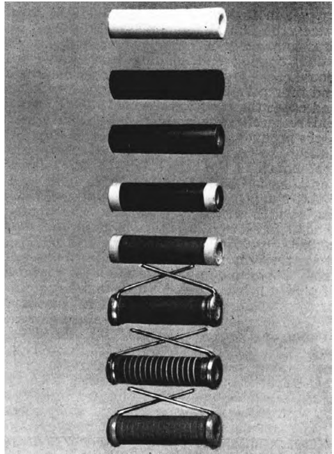
FIGURE 5.1. "Nobleloy" resistors in various stages of manufacture.
