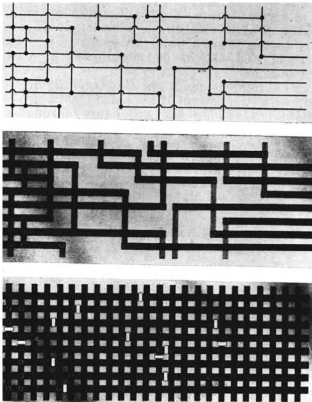
FIGURE 14.1. Development of stamped wiring panel (center) from schematic diagram (top). (Bottom) the same circuit using a standard die.
