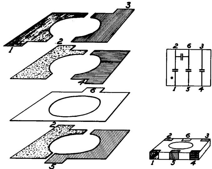
FIGURE 7.2. Arrangement of internal electrodes of four capacitor, S-3 unit.
