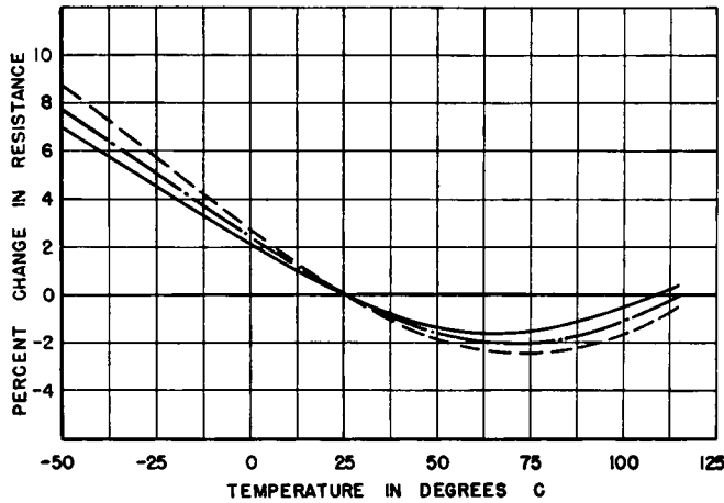
FIGURE 4.5. Temperature characteristic of a given resistance material on phenolic and two different ceramic bodies. — laminated phenolic base, - - - ceramic "S" base, - . . - ceramic "D" base.
