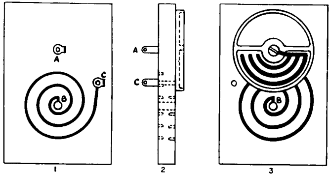
FIGURE 17.5. Drawing showing the construction of the adjustable resonance circuit. (1) Back view; (2) side view; (3) front view.
